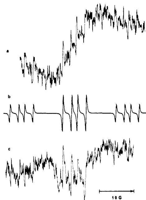
Figure 3. (a) 9.3-GHz EPR spectrum of cyclobutenyl radical 39a at -65 °C in cyclopropane. (b) Computer simulation; see text. (c) 9.3-GHz EPR spectrum of deuteriated cyclobutenyl radical 39b at -65 °C in cyclopropane.
